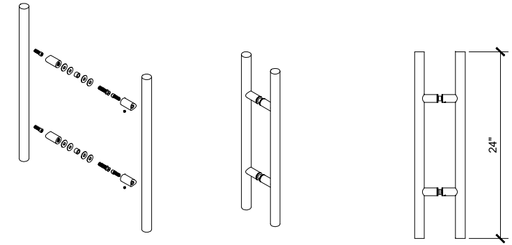
F 24 LADDER PULL RUBY SLIDING DOORS (XO) SCALE: 6"=2'-0"
