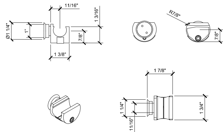
A PLHDSR ANTI-LIFT TOP ROLLER RUBY SLIDING DOORS (XO) SCALE: 6"=1'-0"
