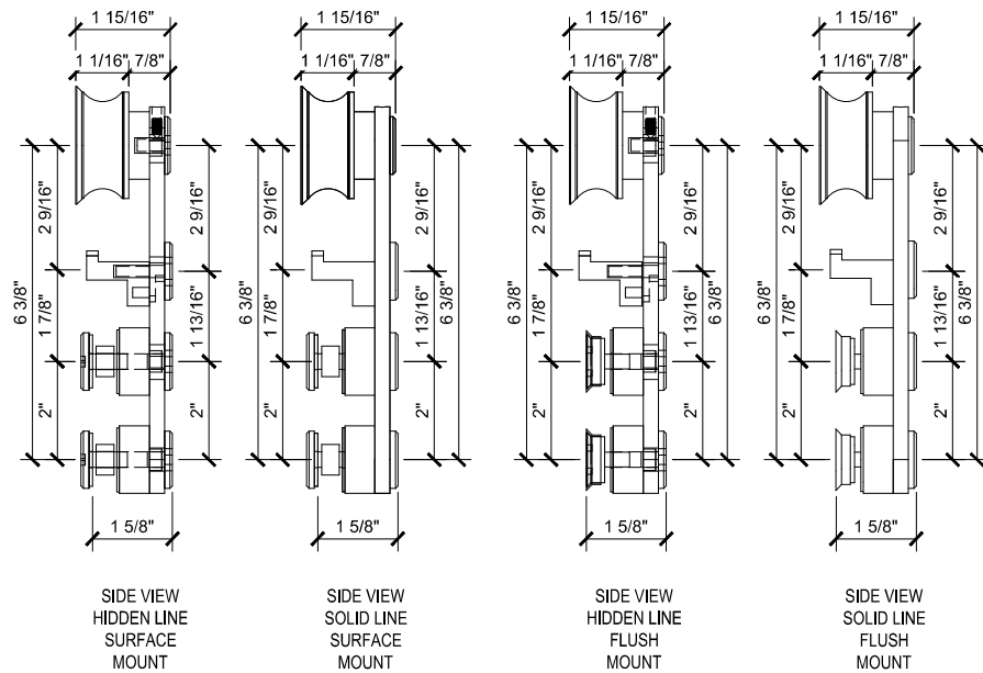
A PLHDSR ANTI-LIFT TOP ROLLER RUBY SLIDING DOORS (XO) SCALE: 6"=1'-0"
